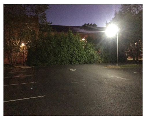
SOLAR AREA LIGHT - 30W, 6000 LUMENS St. Paul's Church, MD - Fixture Height = 15'
