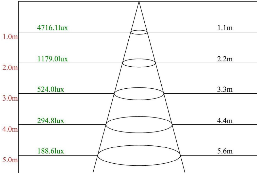
Beam angle of C0plane58.07
